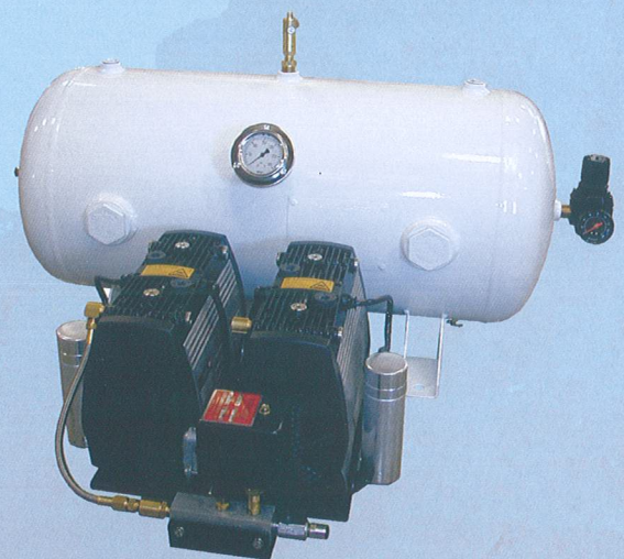
KA-1000 Air Compressor System
